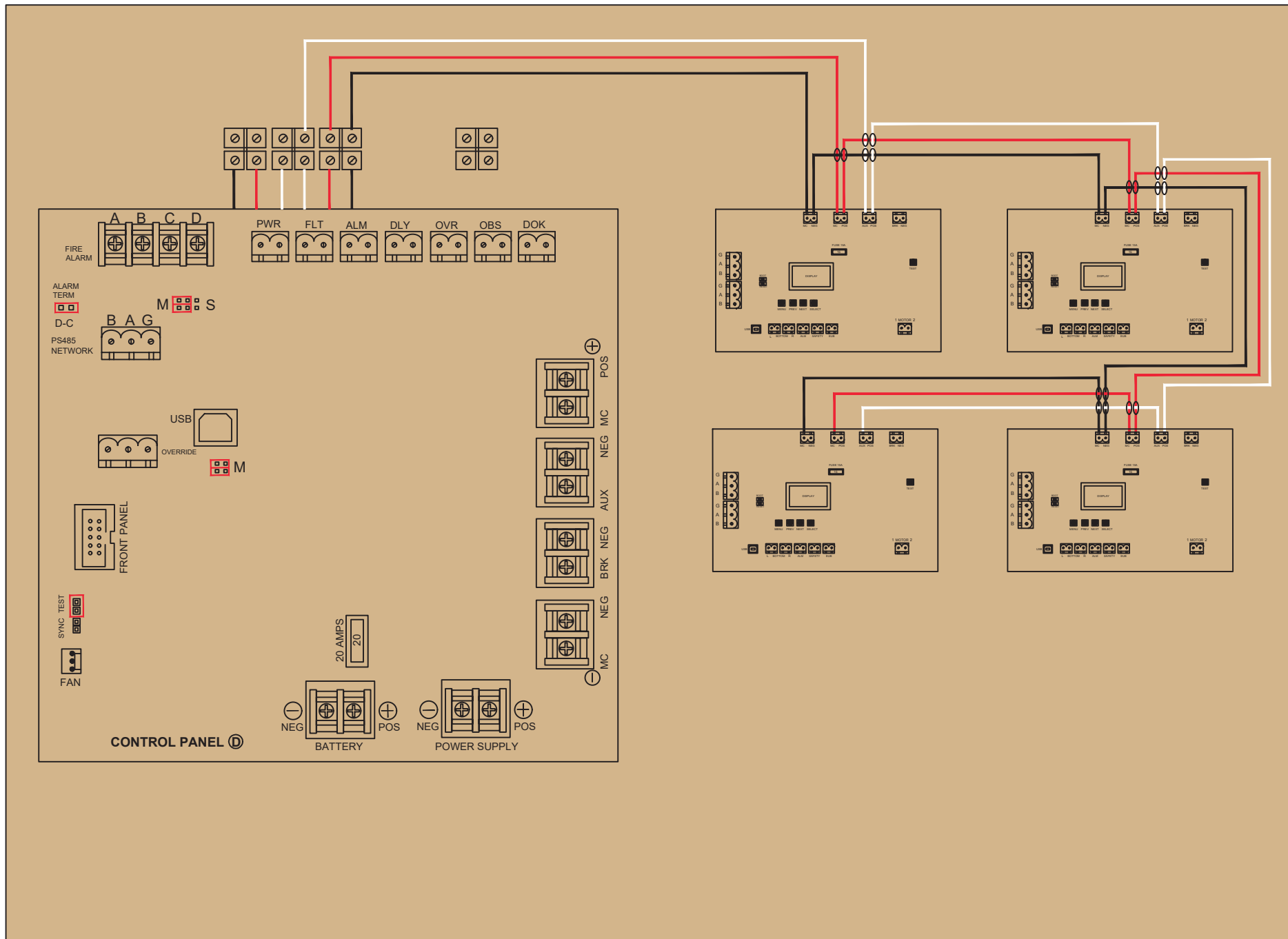
POWER WIRING DIAGRAM. CP TO MC
