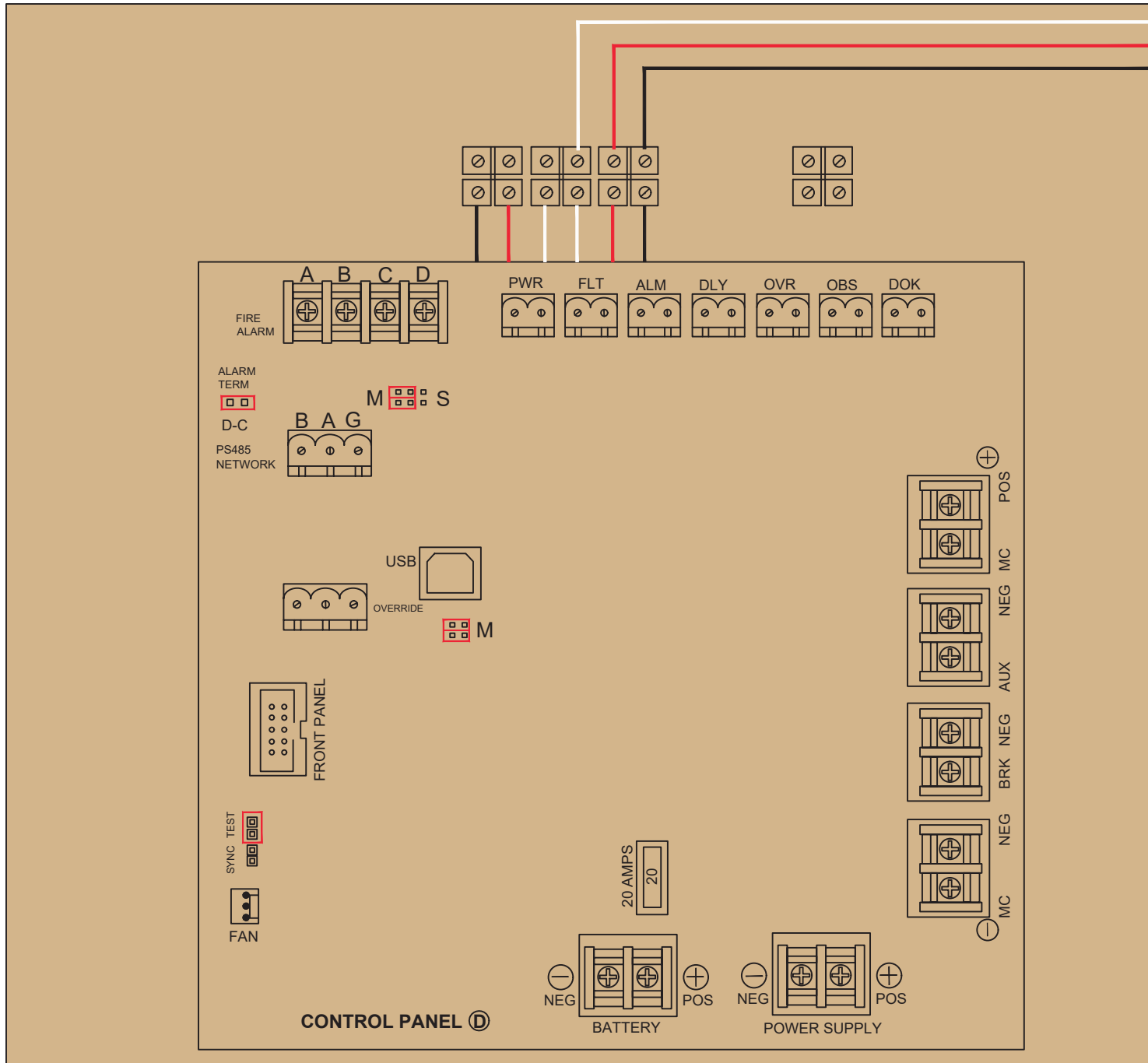
CONTROL PANEL BOARD
