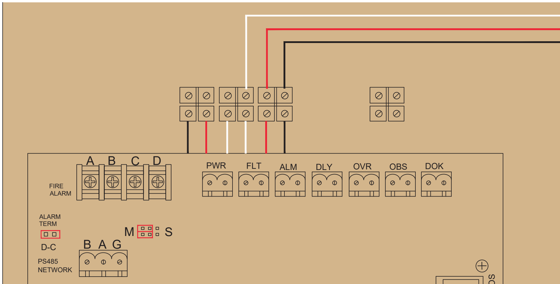
CP POWER WIRING TERMINAL ENLARGED VIEW
